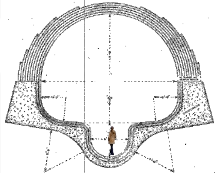
Existing Northeast Boundary Sewer Section (22'-0" x 23'-6")
